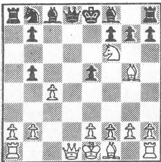
407 After 9 Nxf6
